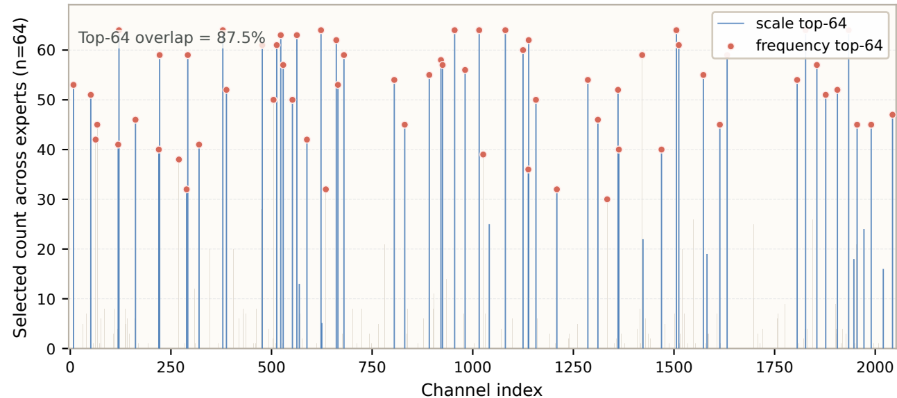
Layer 15 up_proj: top-64 selected-channel frequency
