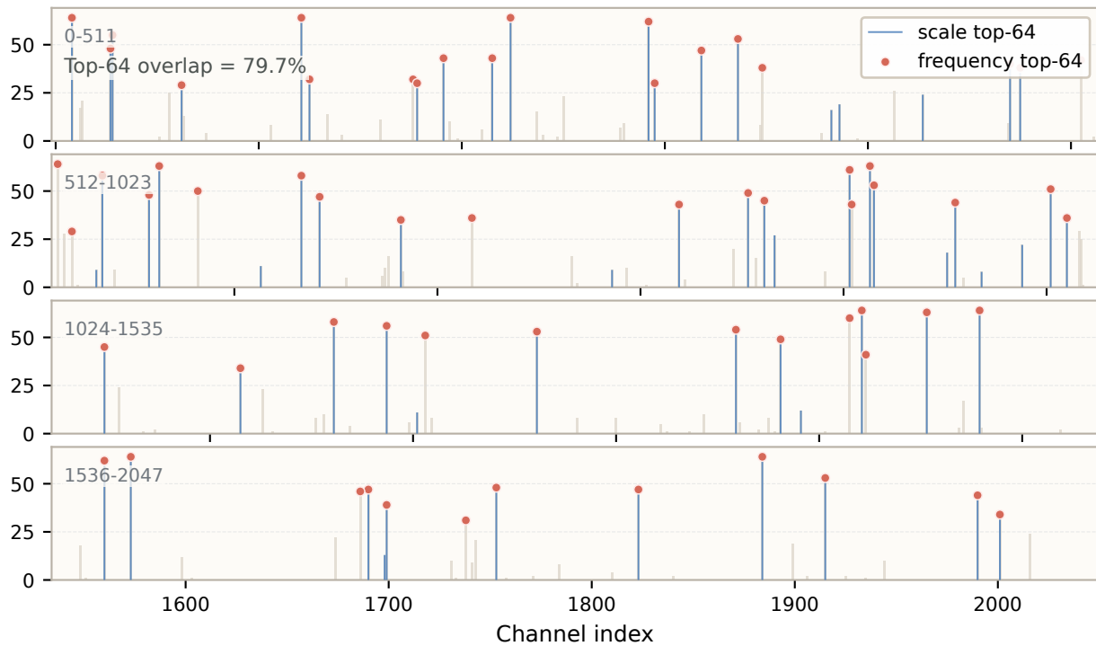
Layer 0 up_proj: top-64 selected-channel frequency
