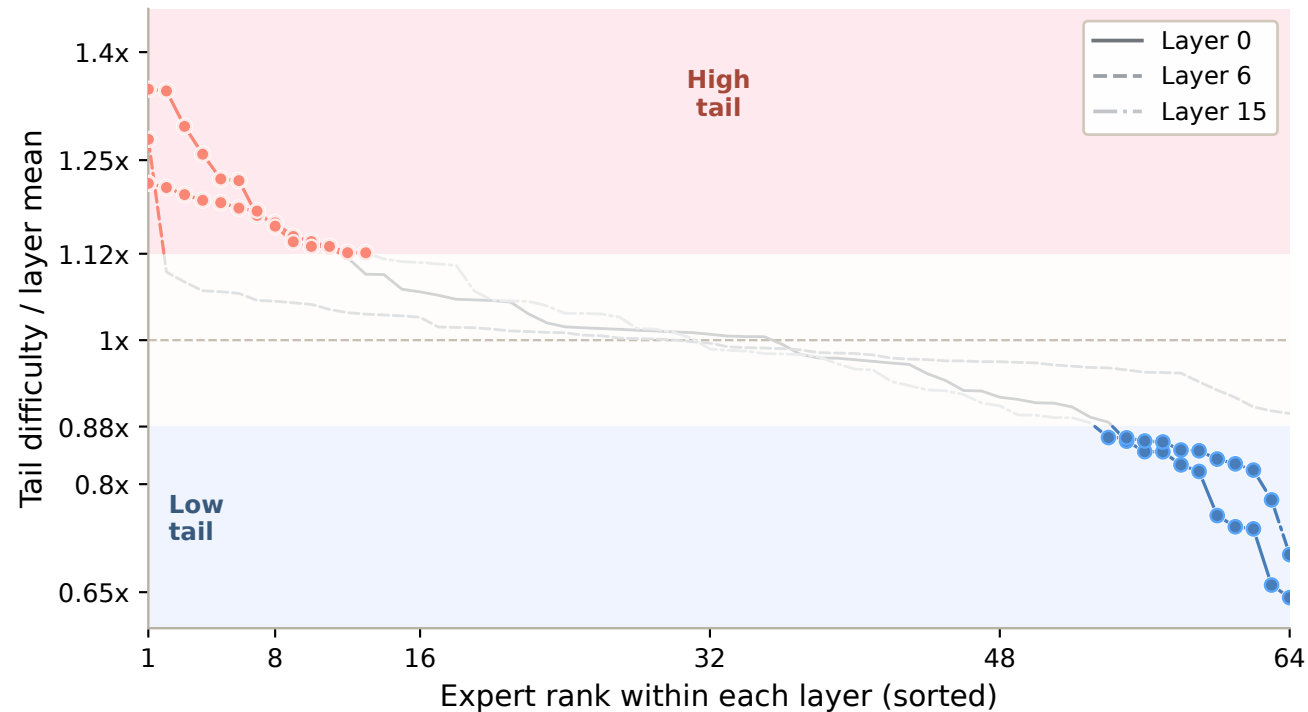
Sorted Expert Tail Difficulty
