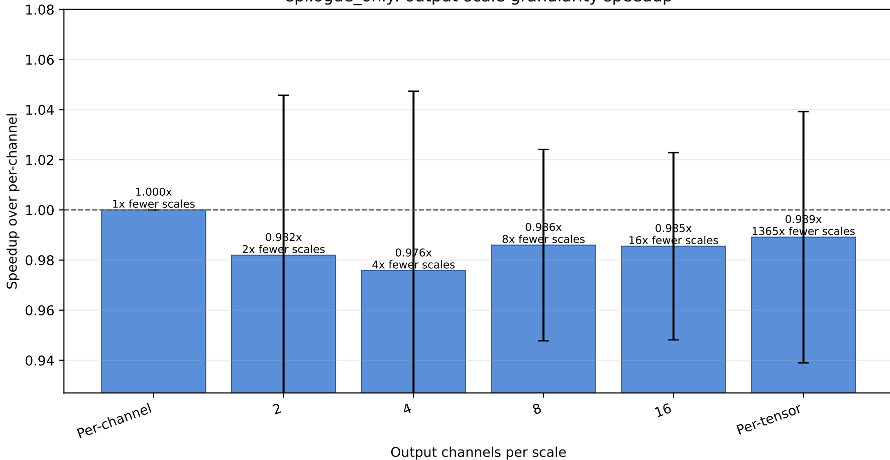
epilogue_only: output-scale granularity speedup
