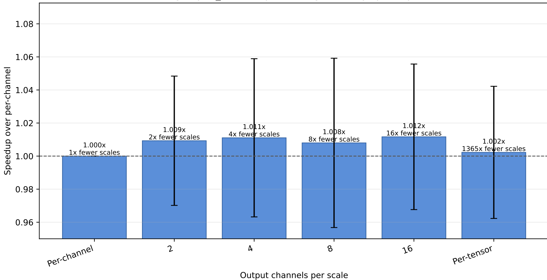
grouped_moe: output-scale granularity speedup
