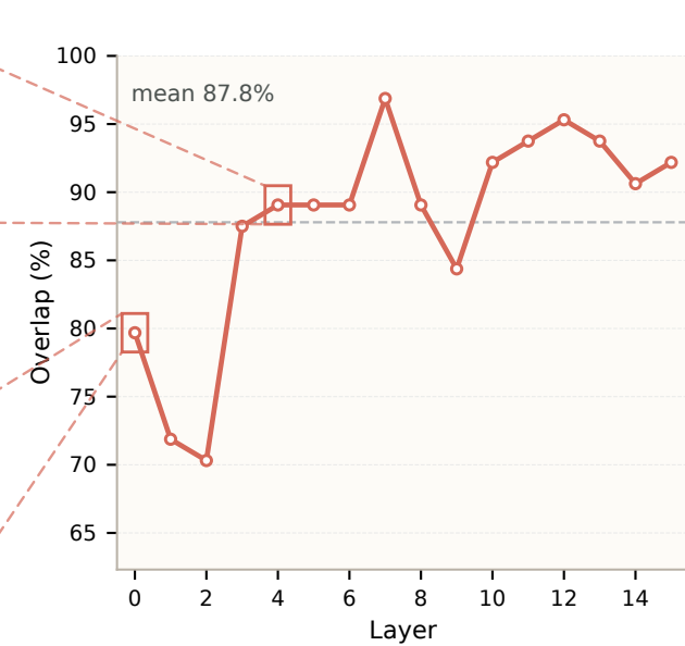
(e) OLMoE layer-wise overlap
