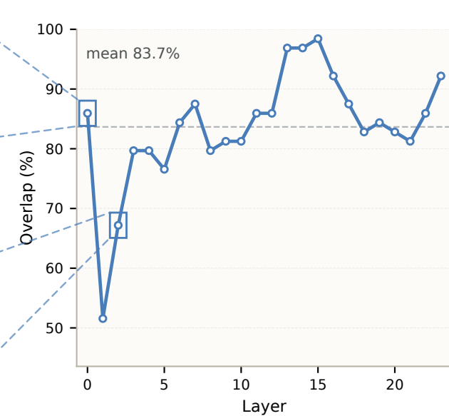
(f) Qwen layer-wise overlap
