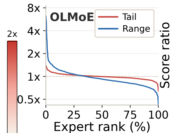
(e) OLMoE sorted score
