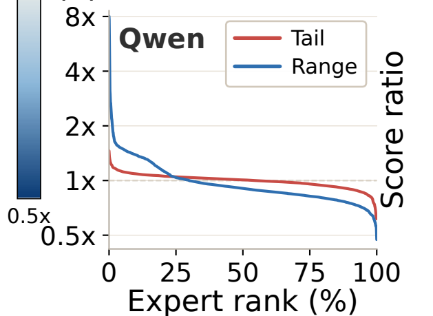
(f) Qwen sorted score
