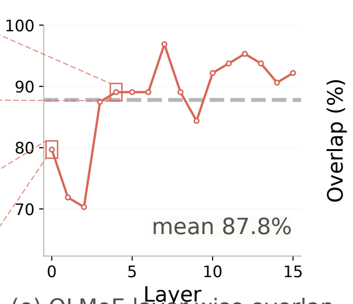
(e) OLMoE layer-wise overlap
