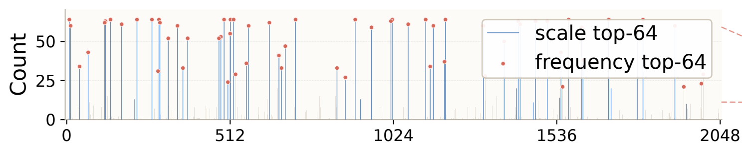
(a) OLMoE L4 overlap 89.1%
