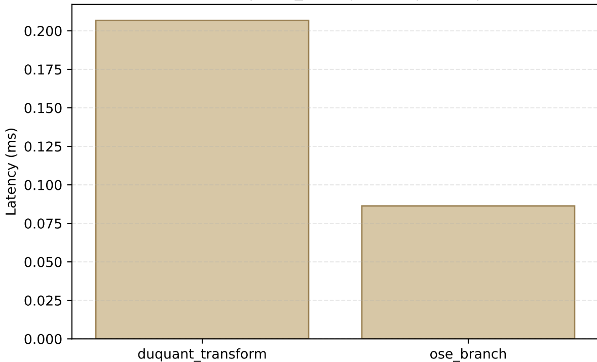
Components | moe_layer | olmoe | E=16 | T=16
