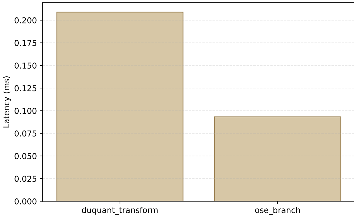
Components | moe_layer | olmoe | E=16 | T=4
