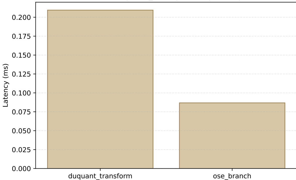
Components | moe_layer | olmoe | E=64 | T=1
