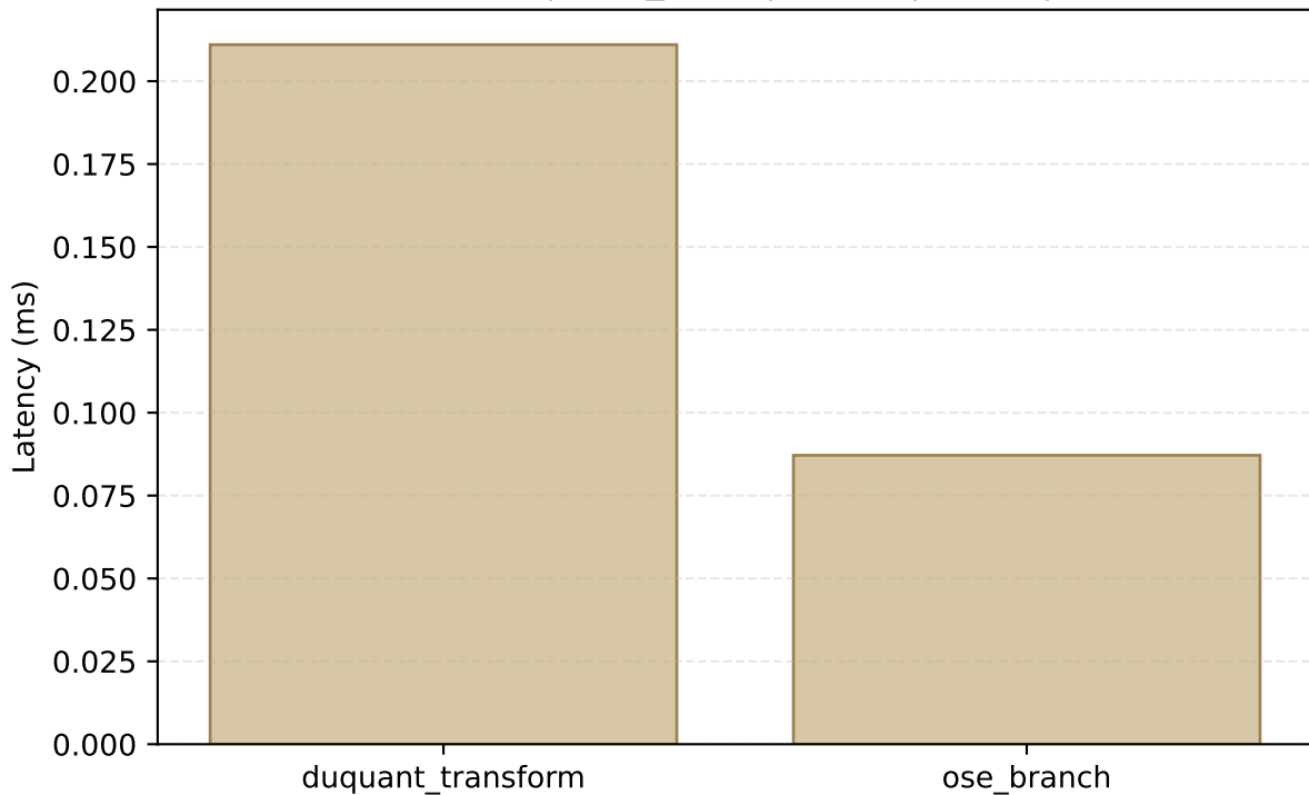
Components | moe_layer | olmoe | E=64 | T=16
