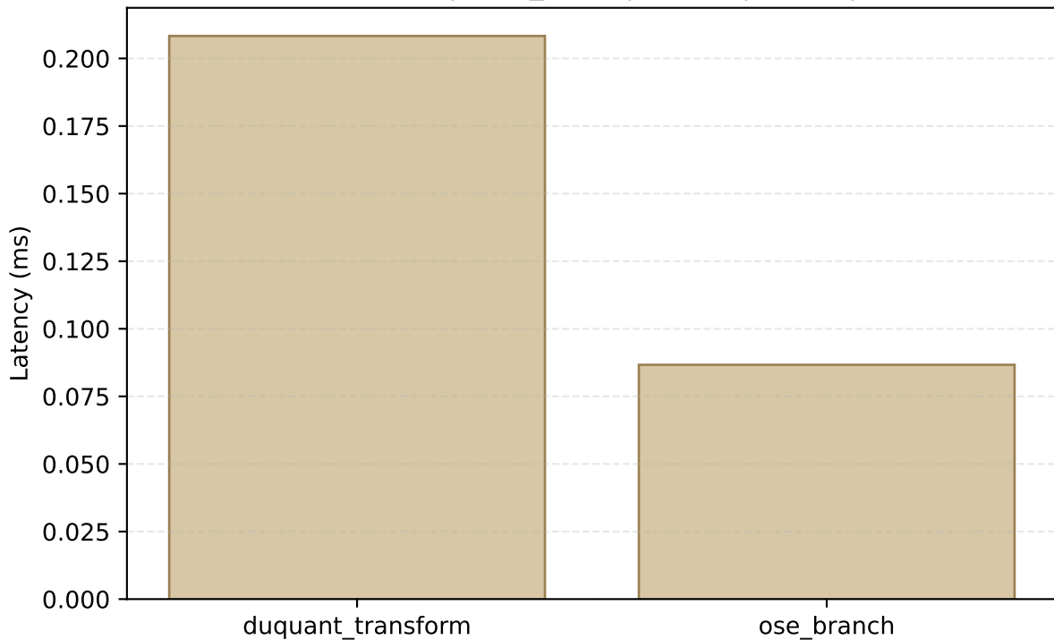
Components | moe_layer | olmoe | E=64 | T=2
