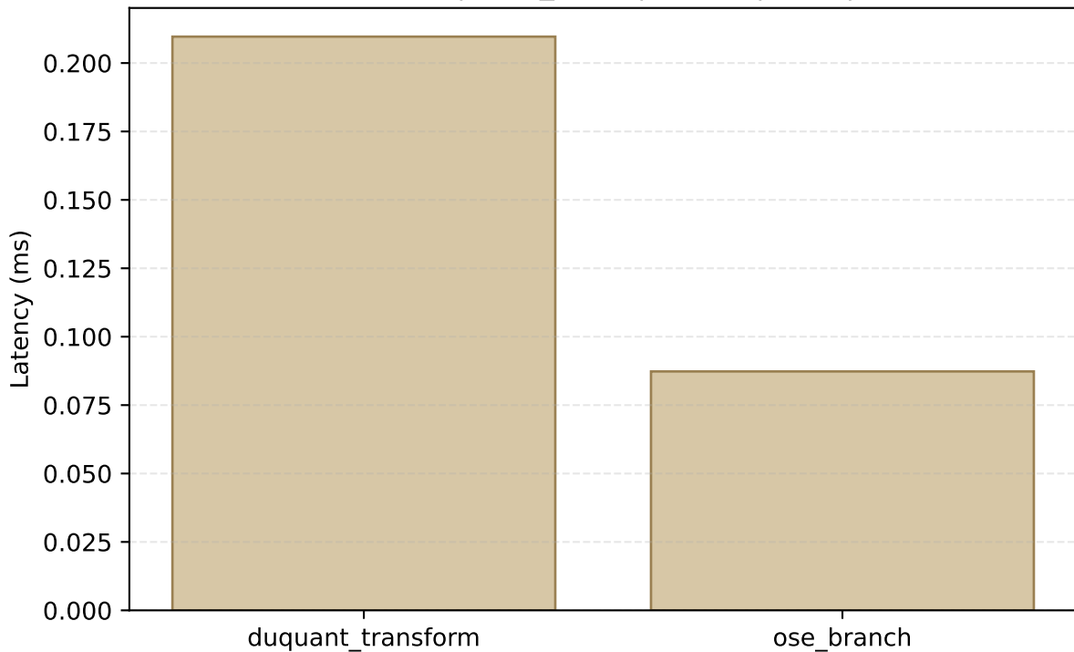
Components | moe_layer | olmoe | E=8 | T=16
