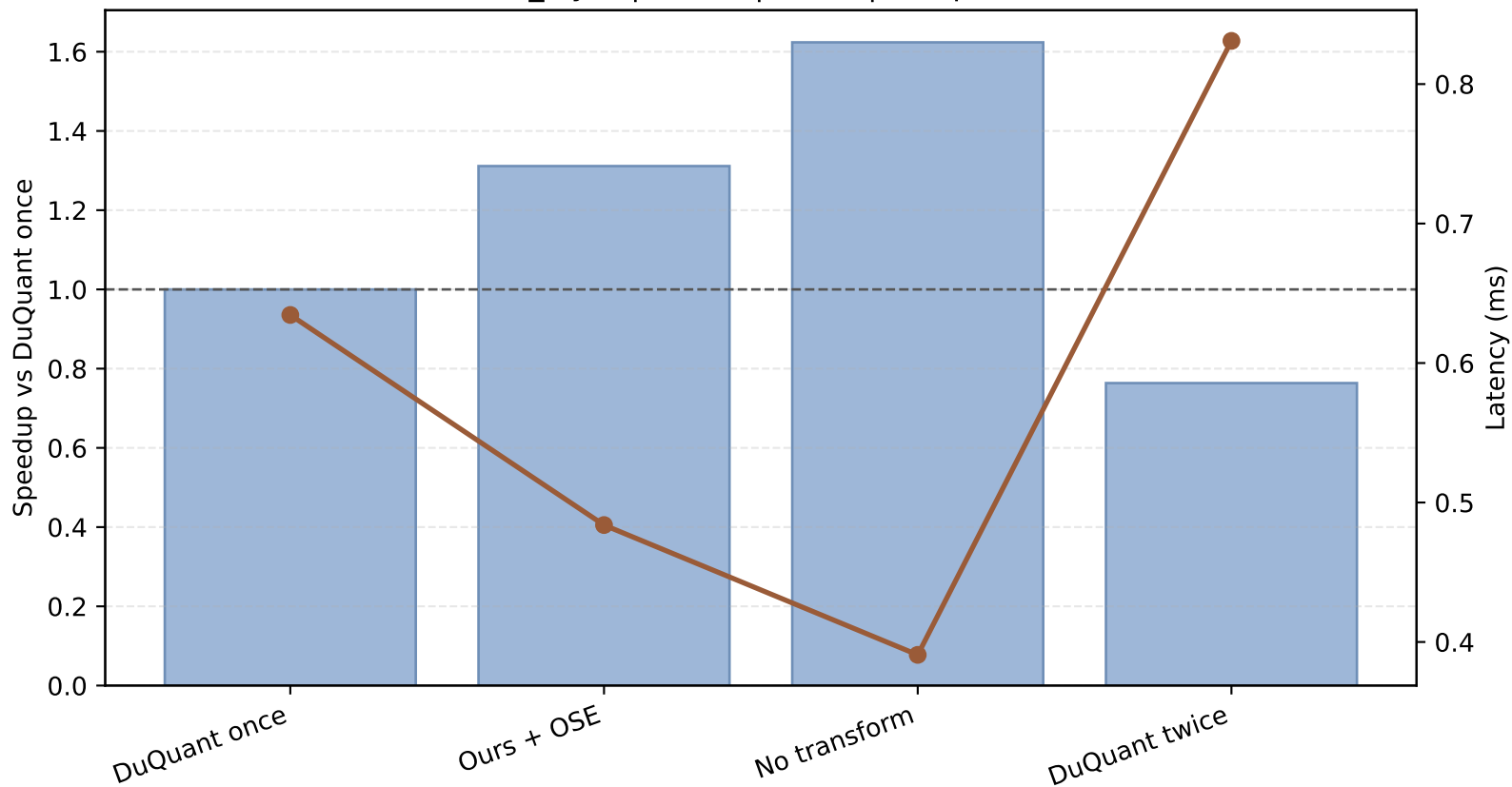
moe_layer | olmoe | E=16 | T/expert=8
