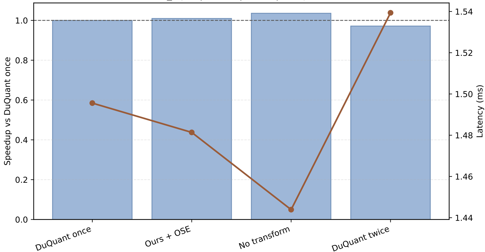
moe_layer | olmoe | E=64 | T/expert=1
