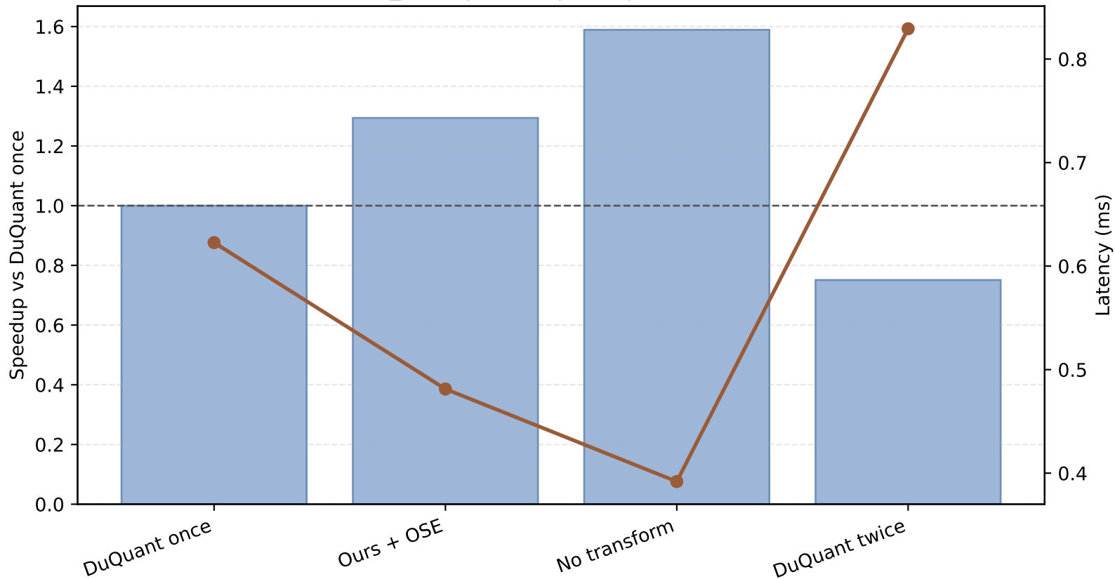
moe_layer | olmoe | E=8 | T/expert=16
