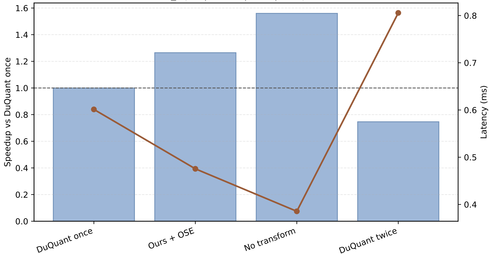
moe_layer | olmoe | E=8 | T/expert=32
