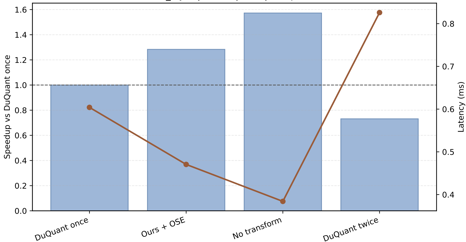
moe_layer | olmoe | E=8 | T/expert=8
