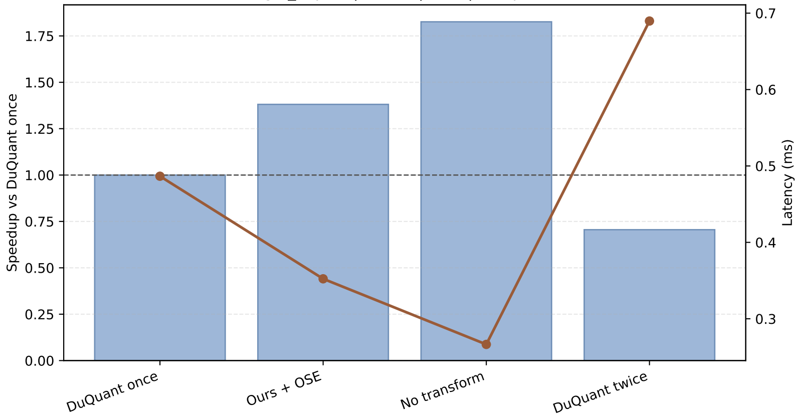
single_expert | olmoe | E=1 | T/expert=4
