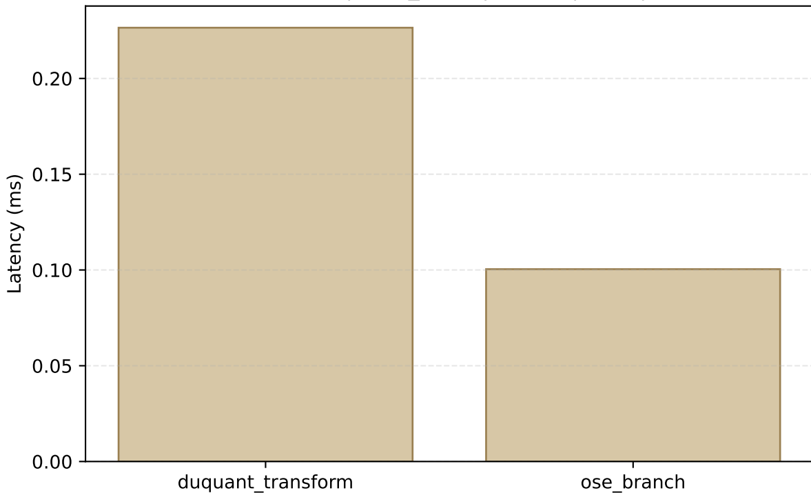
Components | moe_layer | olmoe | E=2 | T=1
