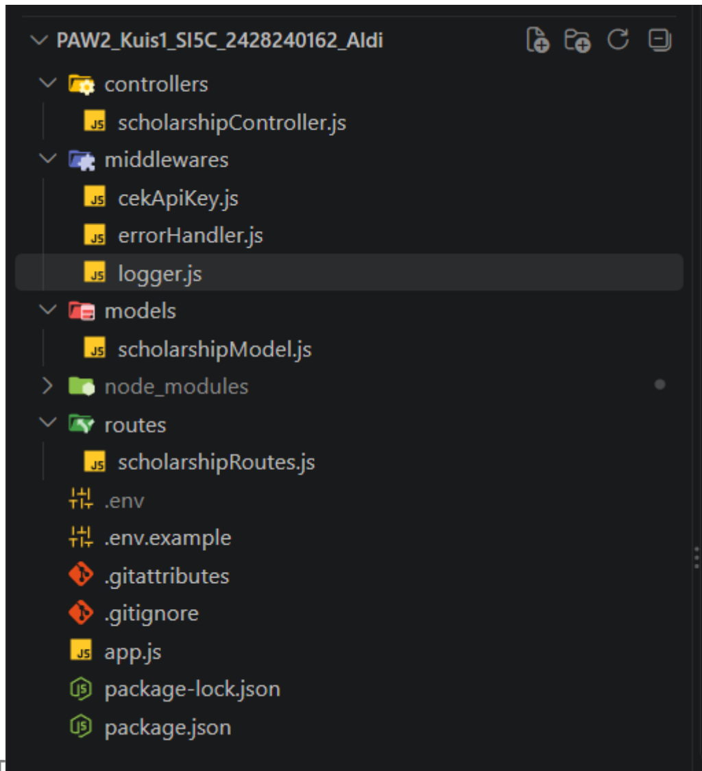
Gambar 2. Struktur folder project
