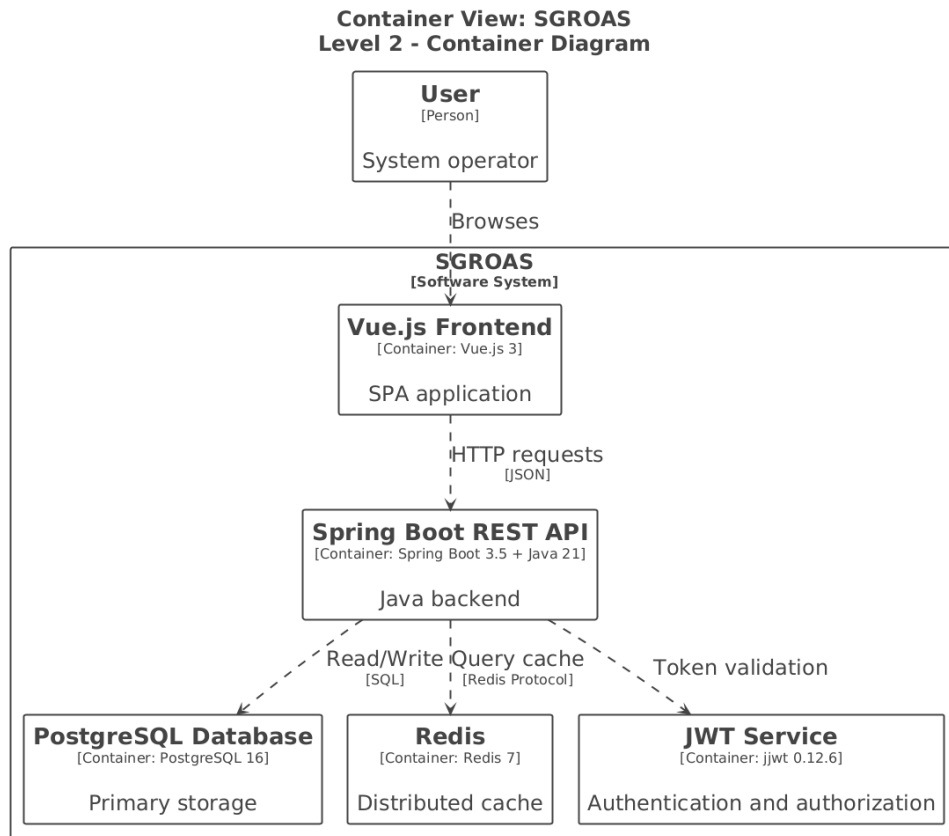
Figura 6.2: C4 Level 2 Diagram — SGROAS System Containers.
