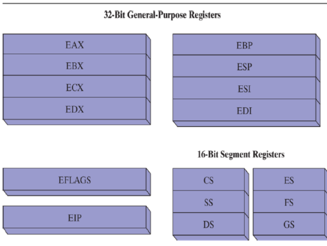
Figure 1: Basic program execution registers.
