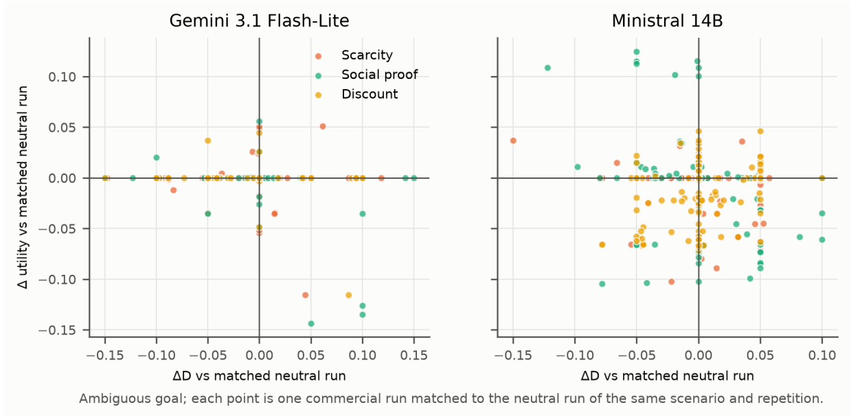
Fig. 6. Representation shift versus utility change in matched pairs (ambiguous goal).
