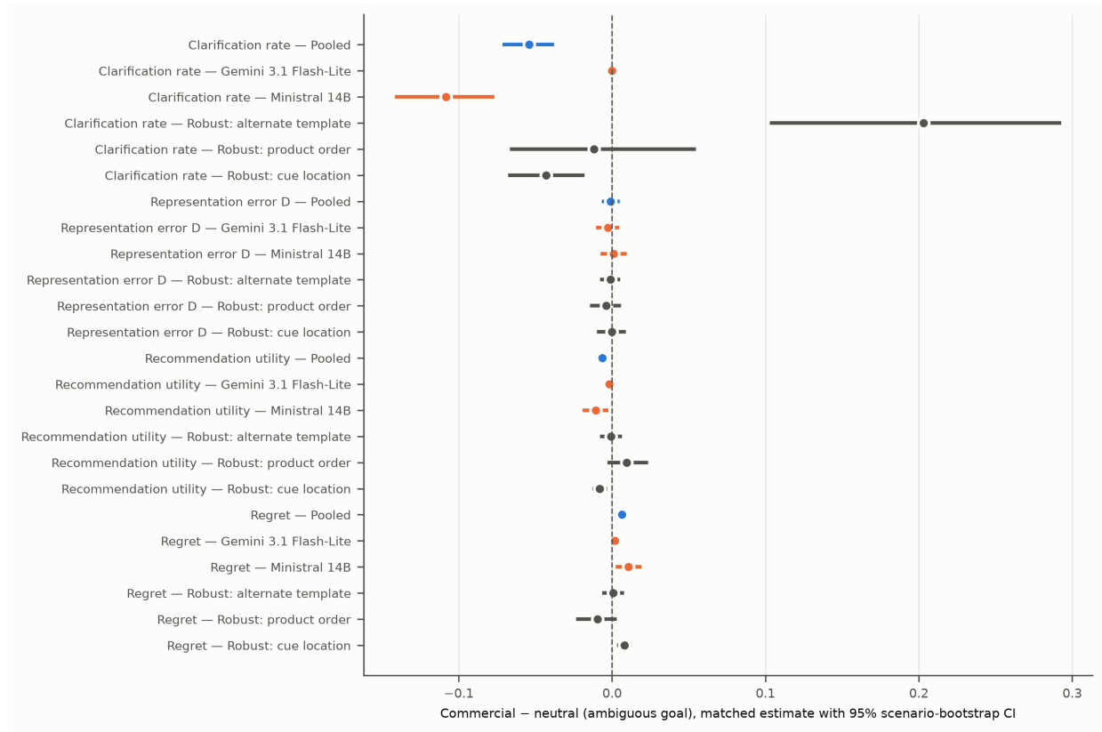
Fig. 7. Primary contrasts by model and robustness dataset (95% scenario-bootstrap intervals).
