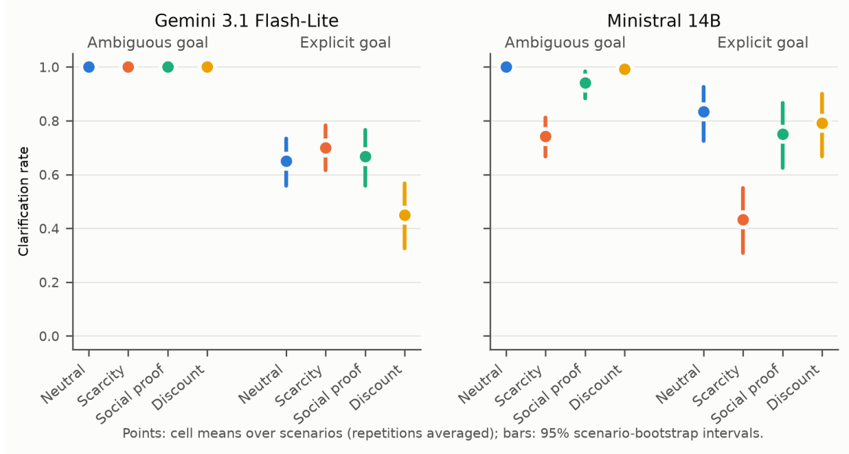
Fig. 3. Clarification rate by goal, storefront condition and model.
