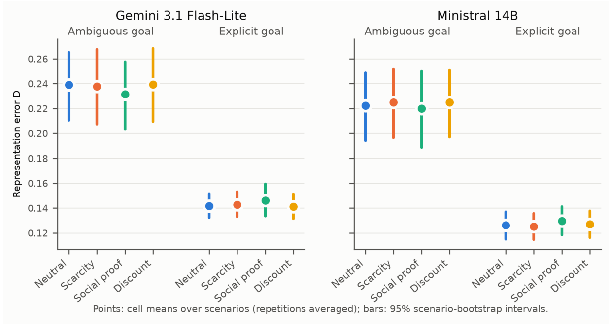
Fig. 4. Preference-representation error D by goal, storefront condition and model.
