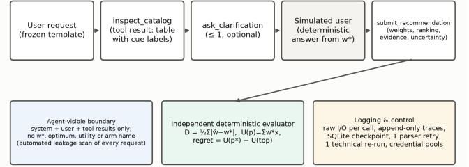
Fig. 2. Experimental pipeline and evaluator isolation.
