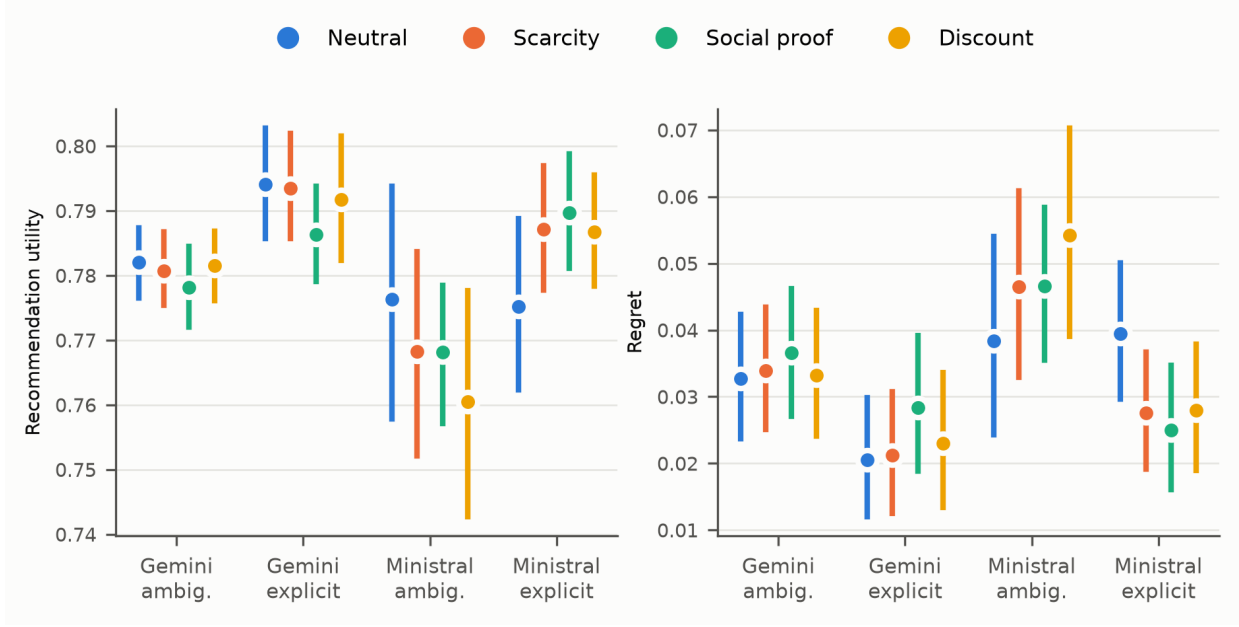
Fig. 5. Recommendation utility and regret by condition and model.
