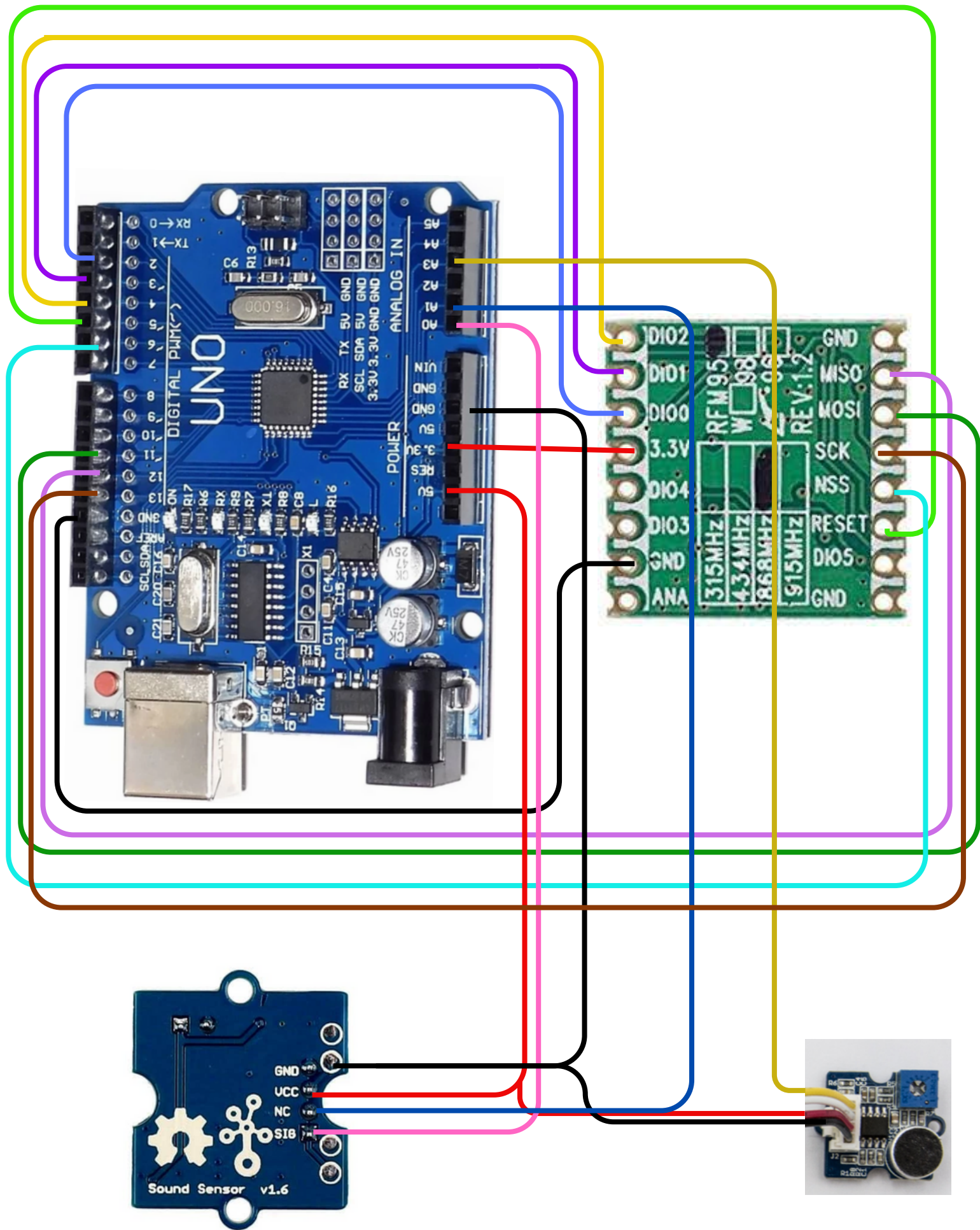
sound sensor
