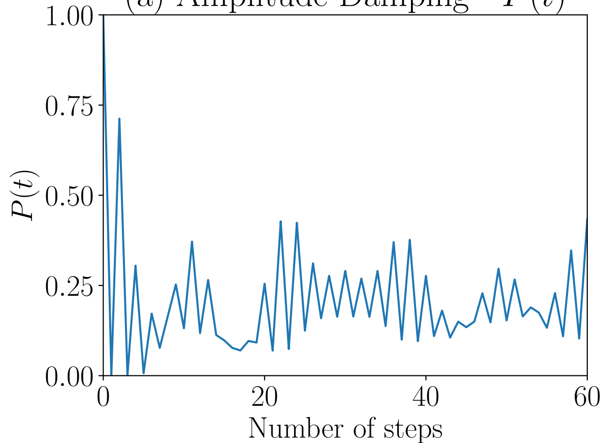
(a) Amplitude Damping - P(t)
