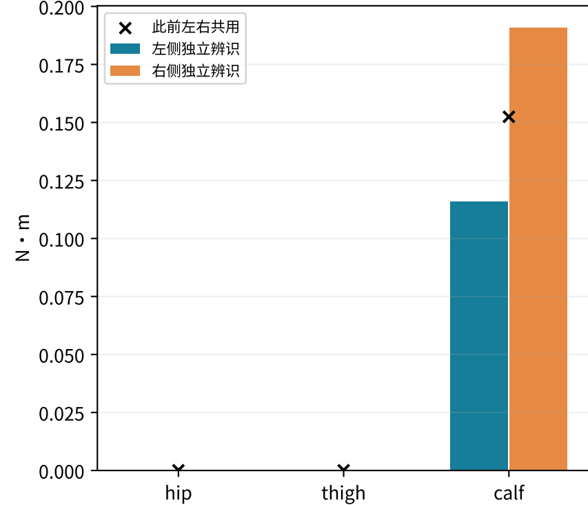
库仑摩擦
