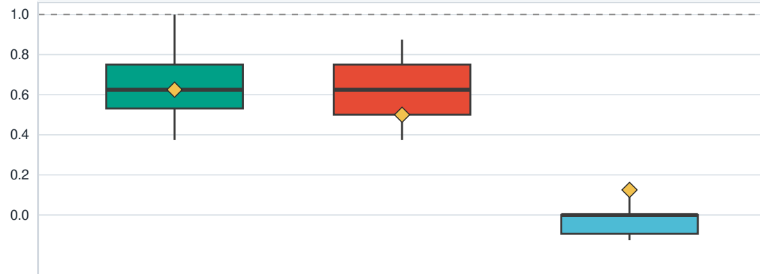
Cohen's kappa
