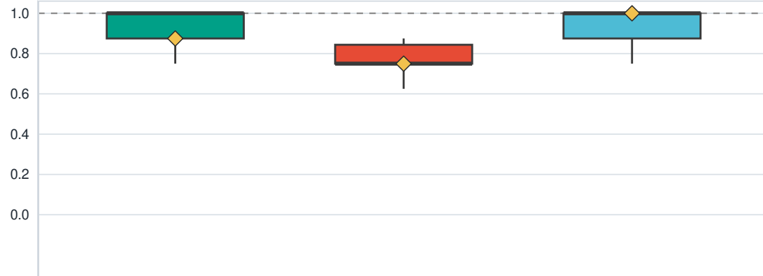
Sensitivity
