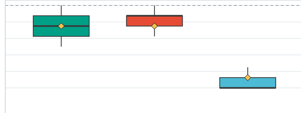
Specificity
