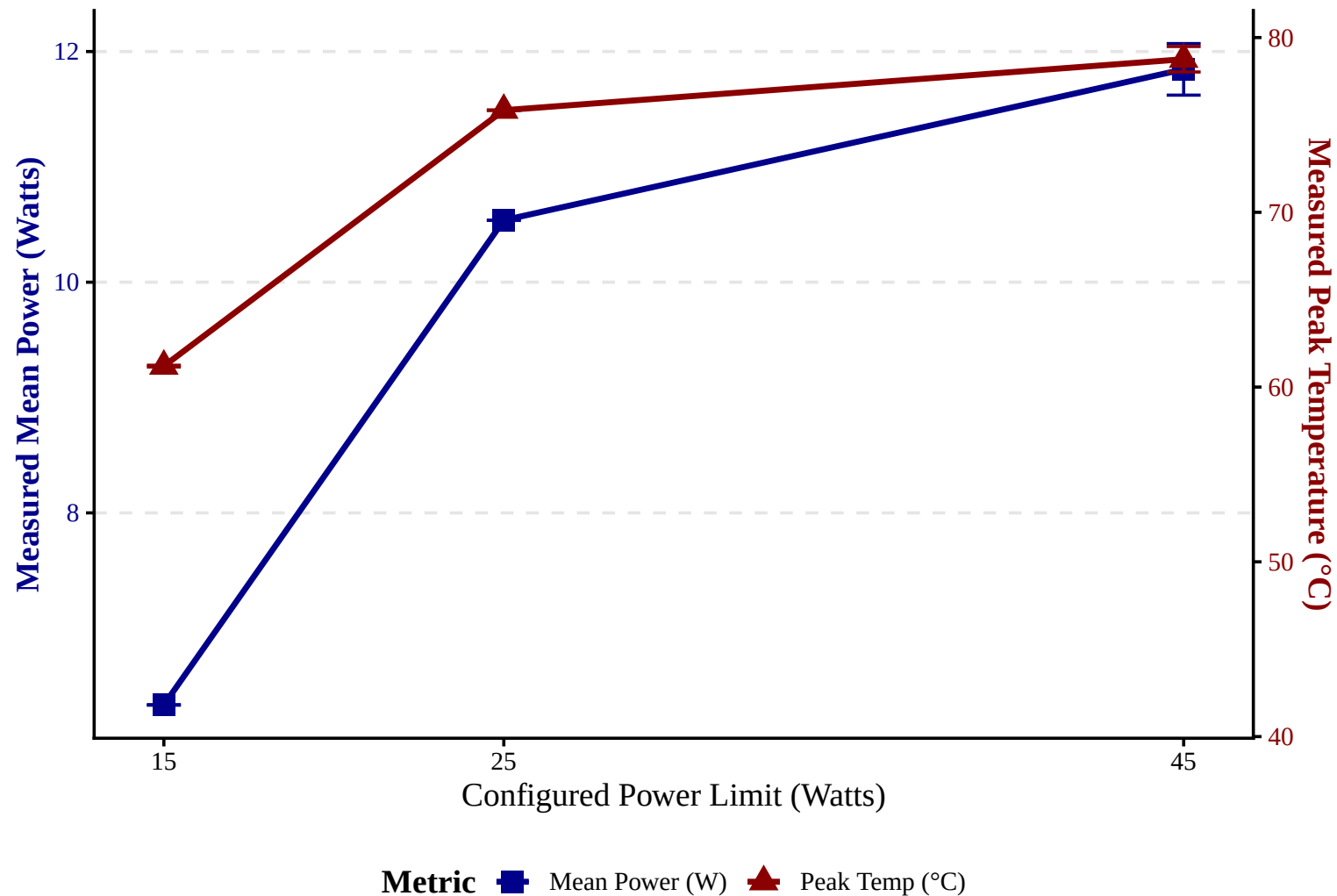
Figure 2: Hardware Validation of Power–Thermal Throttling
