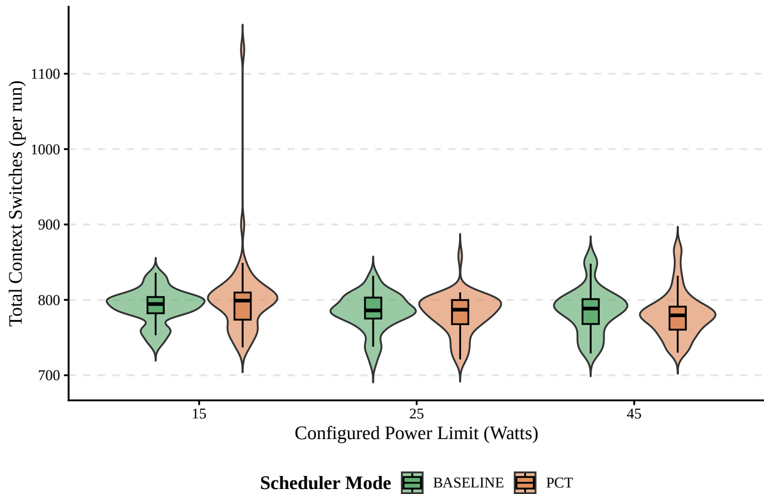
Figure 3: OS Scheduler Interference (Context Switch Density)
