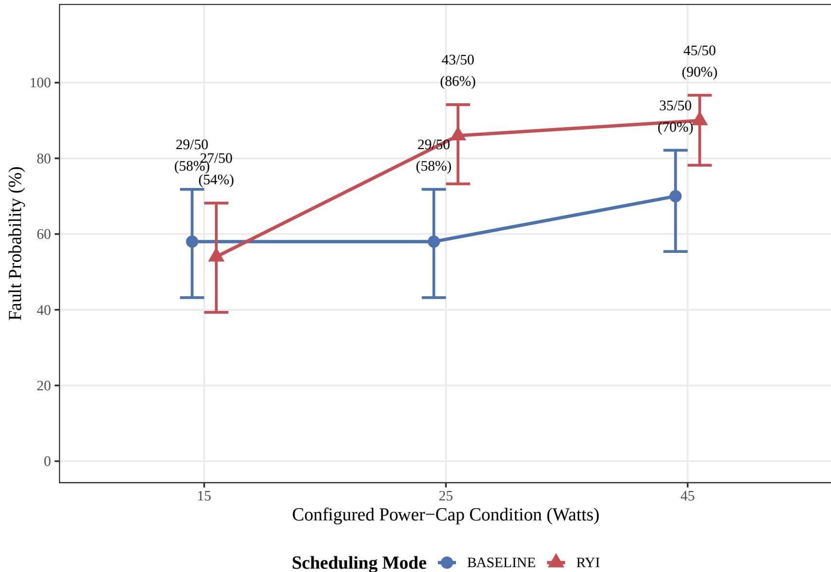
Figure 1: Concurrency Fault Manifestation Rate (with 95% Binomial Confidence Intervals)
