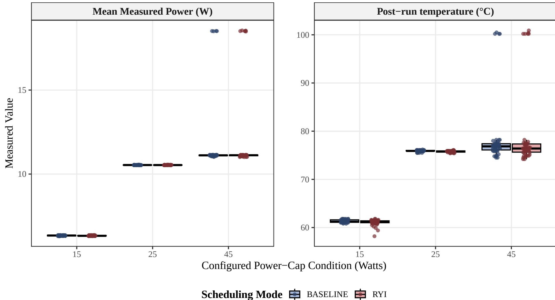
Figure 2: Thermal and Measured-Power Validation
