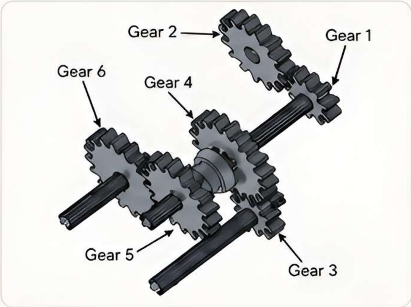
Isometric View (Gears 1-6)
