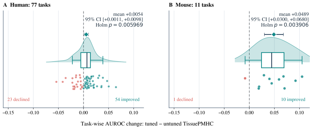
Fig. S5: Task-wise change in fixed-test AUROC after training-only hyperparameter tuning. Each point is the difference between tuned and untuned TissuePMHC after first averaging the same task over seeds; positive values favor the tuned configuration. Open diamonds show the mean change, and horizontal bars show 95% intervals from 10,000 bootstrap resamples of complete tasks. Two-sided paired Wilcoxon signed-rank tests were performed separately for Human and Mouse, then adjusted together by Holm’s method (Human: 77 tasks, mean +0.0054, 54 improved, adjusted p = 0.0060 ; Mouse: 11 tasks, mean +0.0489, 10 improved, adjusted p = 0.0039 ). The intervals and tests describe this internal fixed-test task inventory and are not biological-replicate or cohort-level inference.
