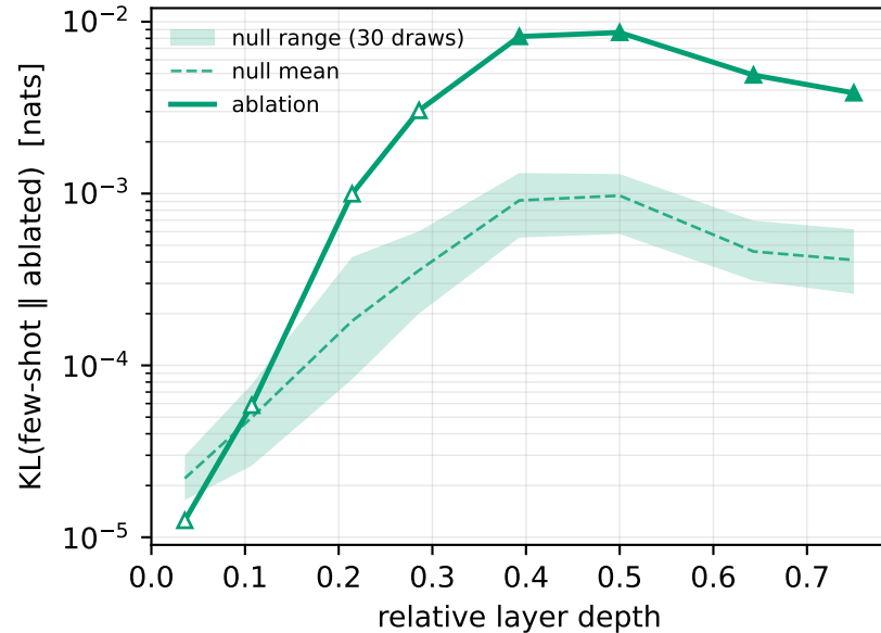
(c) MMLU: ablation vs. null
