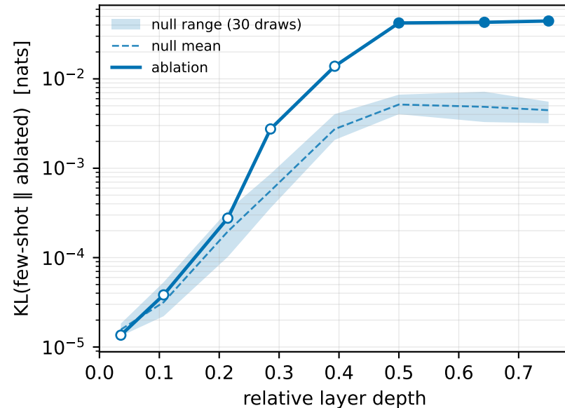
(a) Arithmetic: ablation vs. null
