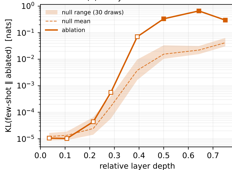
(b) Entity: ablation vs. null
