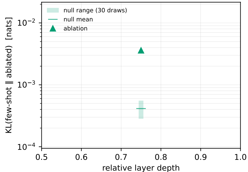
(c) MMLU: ablation vs. null
