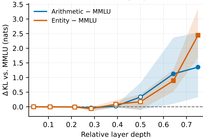
Residual-ablation KL, group – MMLU
