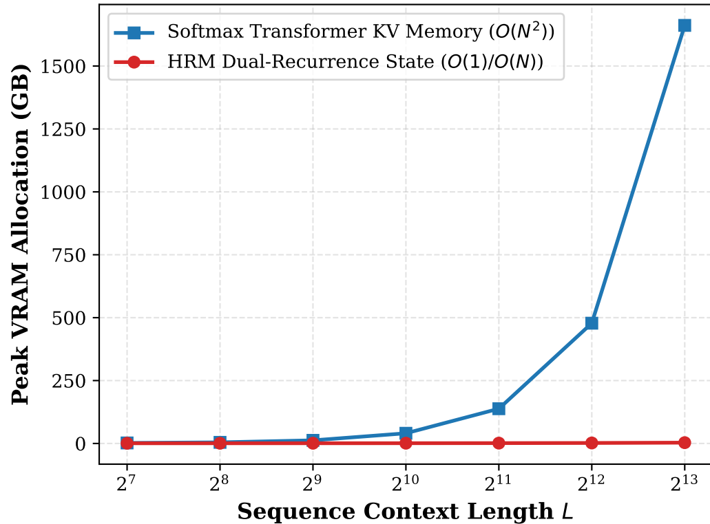
Context Length vs VRAM Footprint
