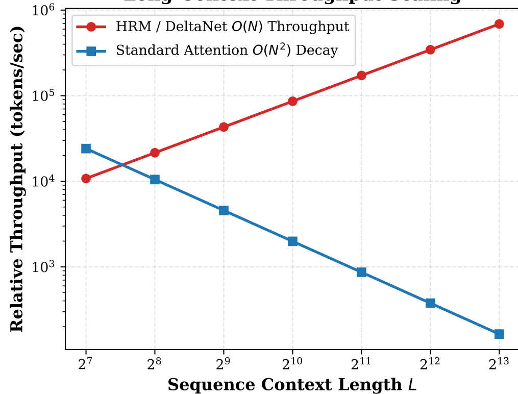
Long-Context Throughput Scaling
