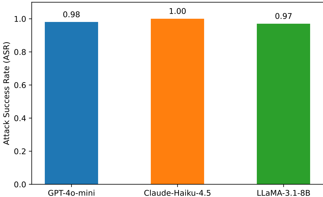
ASR on HotpotQA Dataset
