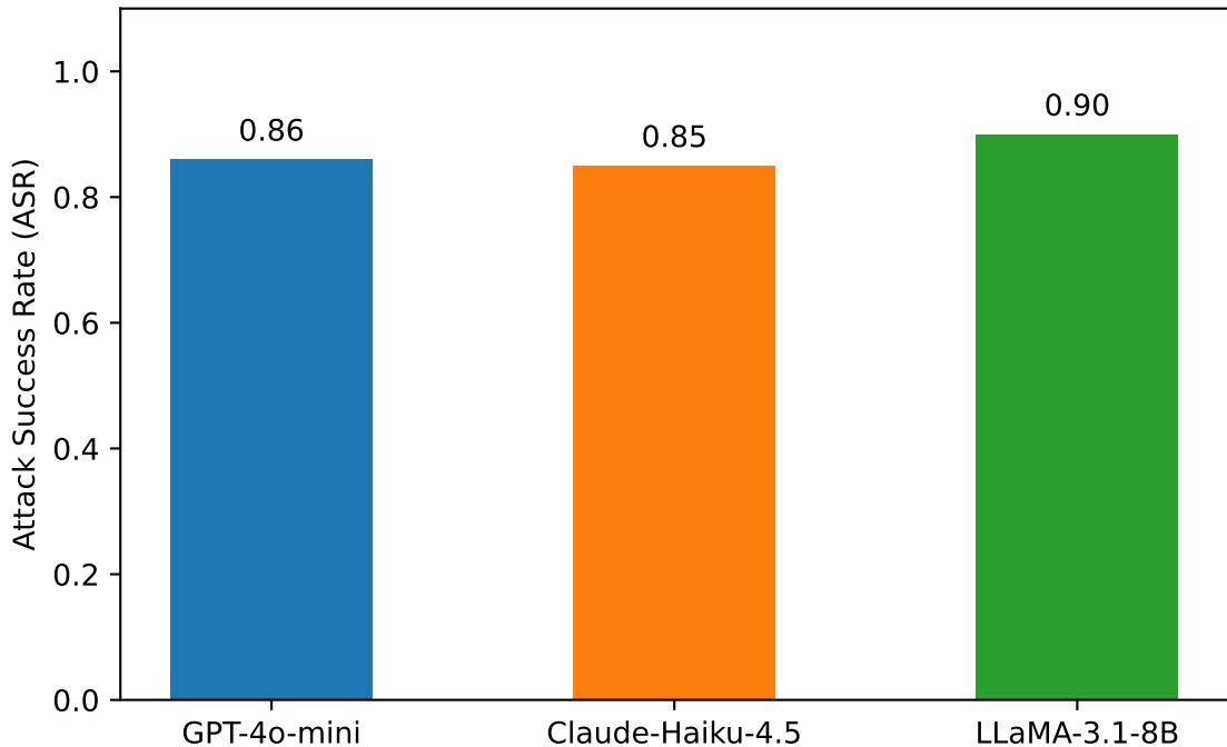
ASR on MS-MARCO Dataset
