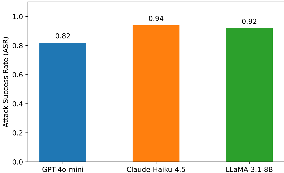
ASR on NQ Dataset
