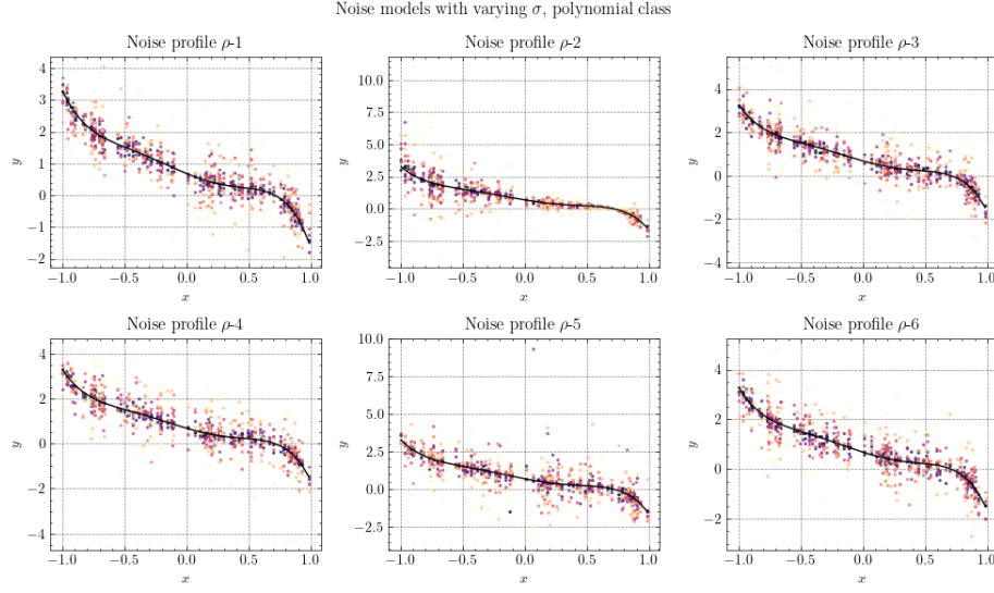
Figure 4.4: The different variations of the noise profile that can be often seen when sampling from a polynomial model, particularly constrained, 5th degree p_5 univariate polynomial on [-1, 1] domain inverse range. By order, (1) represents mean-scale additive noise, (2) considers heteroskedastic multiplicative noise, (3) considers variance-scaled additive noise, (4) considers absolute additive noise (where scale independent of y ), (5) considers heavy-tailed noise (Student- t modelling), and (6) is the standard canonical Gaussian noise (basically the default). We can see that each distributive pattern produces various different, often irreducible to Gaussian noise configurations.
