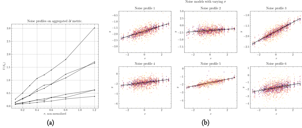
Figure 4.3: Noise uncertainty creation, aggregated through the metric U(S'_n) of the diffused dataset. Here, we can see that for y -only corrupted noise, the uncertainty increased on bounding for 2\sigma^2 , of which diverges several noise profiles from one another. An interesting outlier is in the suppressing effect of mean-scale additive noise, which is not as expected.
