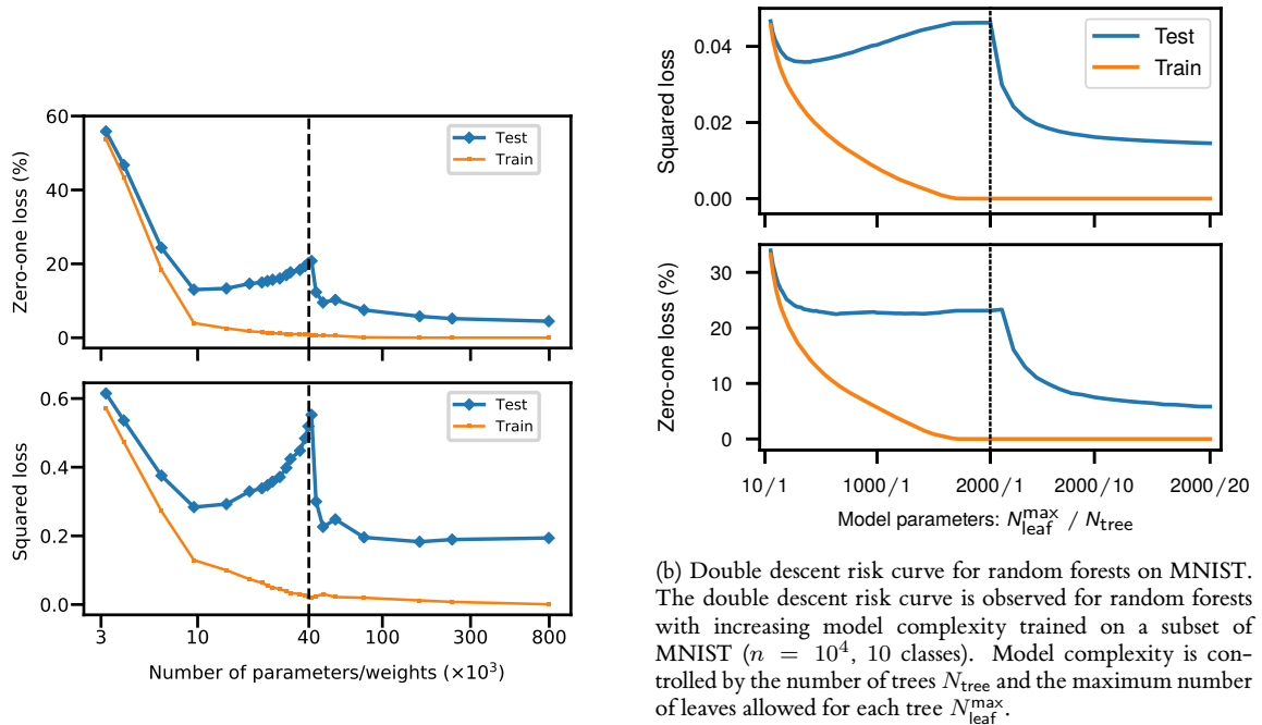
(a) Double descent risk curve for a fully connected neural network on MNIST. Training and test risks of a network with a single layer of H hidden units, learned on a subset of MNIST ( n = 4 \cdot 10^3 , d = 784 , K = 10 classes). The number of parameters is (d + 1) \cdot H + (H + 1) \cdot K . The interpolation threshold (black dotted line) is observed at n \cdot K . Taken from Belkin et al. [2019a].
