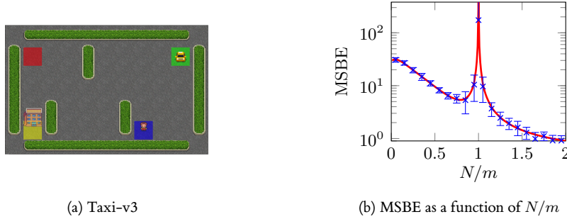
Figure 3.8: As the model complexity N/m (for N parameters, m distinct visited states) increases, the MSBE first shows a U-shaped curve, peaking around the interpolation threshold ( N = m ). Double descent refers to the phenomenon for N/m > 1 where the MSBE drops once again. Continuous lines (red) indicate the theoretical values, the crosses (blue) are numerical results averaged over 30 instances with their standard deviations after the learning with regularized LSTD on Taxi-v3 for \gamma = 0.95 , \lambda = 10^{-9} , n = 5000 , m = 310 . Taken from Brellmann et al. [2024]
