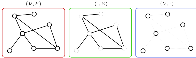
Figure 4.11: Illustrative decomposition of the graph on its simplexes edges and vertices: Each of the decomposed space \mathcal{V} and \mathcal{E} can be encoded separately to their own ordeal, for example, of the edge connection through incident matrix.
