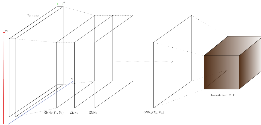
Figure 4.12: A conceptual illustration on the running flow of an n -layer GNN on particular structure of interest. Note that the data section itself has particular embedding structure on its own.
