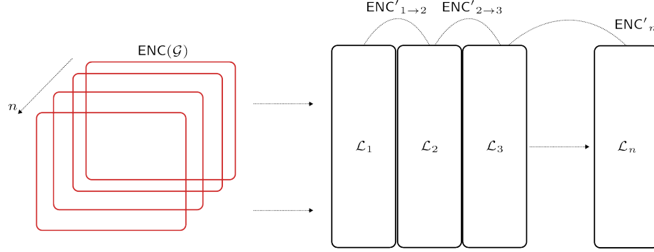
Figure 4.13: Encoding space and the change of encoding inbetween a static graph (or snapshot-wise) GNN. The encoding space is warped toward arbitrary notions inside a GNN, to the point that after certain layers of processing, the encoding outputs different from expected encoding space (native to the model, not to the designer), though there might be universal notions preserved, like the degree of node represented in a different way.
