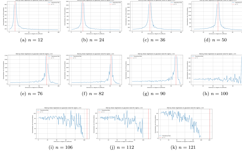
Figure 4.5: Theorem 4.3.1 behaviours on randomized setting. For this model, we have d = 100 , \sigma = 0.5 , and variational n . Full test cases are for p = [1, 100] , n = \{12, 24, 36, 50, 76, 82, 90, 100, 106, 112, 121\} accordingly. The test function of the concept itself is the same linear model, but with different input only.
