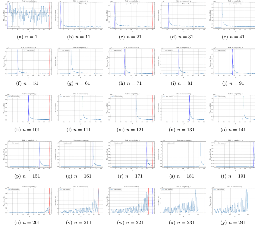
Figure 4.9: Extension general experimentation, using the prediction made of theorem 4.3.1 for verification. Here, q = 1 as the general basis case of verification.
