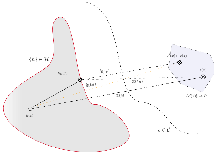
Figure 2.1: An illustration of statistical learning theory on the evaluation of the risks and errors, during learning process. c' is presented in the 'orbital' vicinity around c , with its distance of certain metric define how 'accurate' the reconstruction from distribution can be. Of the hypothesis set \mathcal{H} , there exists the Bayes hypothesis h_B and an arbitrary 'random' hypothesis h , and their respective measure.
