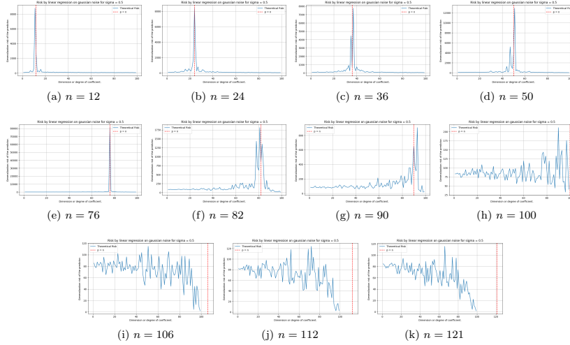
Figure 4.6: Contrary to Theorem 4.3.1, this is the behaviours on randomized setting for standard parameter-wised mean square error measure (MSE-on-parameter). For this model, we have d = 100 , \sigma = 0.5 , and variational n . Full test cases are for p = [1, 100] , n = \{12, 24, 36, 50, 76, 82, 90, 100, 106, 112, 121\} accordingly. The test function of the concept itself is the same linear model, but with different input only.
