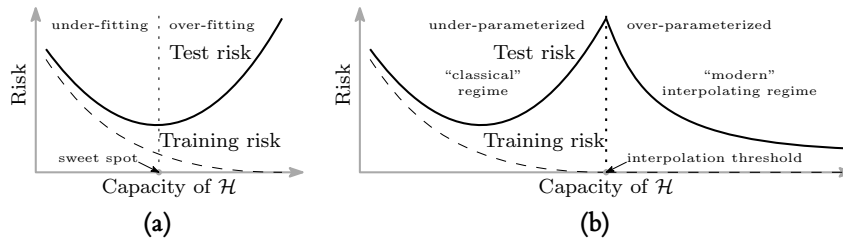
Figure 3.5: Curves for training risk (dashed line) and test risk (solid line). (a) The classical U-shaped risk curve arising from the bias-variance trade-off. (b) The double descent risk curve, which incorporates the U-shaped risk curve (i.e., the “classical” regime) together with the observed behaviour from using high capacity function classes (i.e., the “modern” interpolating regime), separated by the interpolation threshold. The predictors to the right of the interpolation threshold have zero training risk. Reproduced from Belkin et al. [2019a] .
