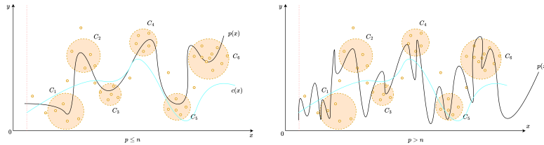
Figure 6.4: Intuition of Hypothesis 6.6.1. Effectively, in the overparameterized range ( p > n ), the problem turns into soft interpolation, where the polynomial is possible to be dense enough such that relative error remains internally low. This can also happen if the dataset itself is intrinsically large.
