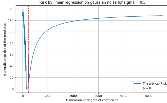
Figure 4.8: Similar experiment according to setting and result of Theorem 4.24, where p is in the range [1, 5523] . Here, we can see small double descent modelled exactly at the interpolation threshold, while the later region exhibit similar phenomenon as bias-variance tradeoff.
