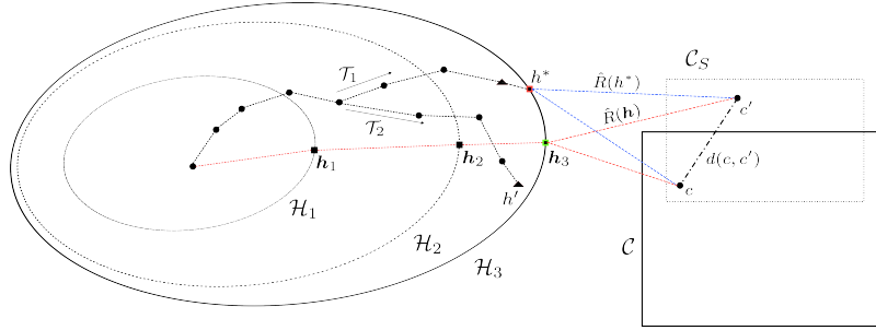
Figure 6.1: Illustrative dynamic of the learning problem. For an incremental hypothesis space sequence \mathcal{H}_1, \mathcal{H}_2, \mathcal{H}_3 , we aim to obtain the procedure \mathcal{T} that would either reach the generalization solution h , or the empirical solution h^* for a particular hypothesis class, with respect to the concept c and its observed concept c' . Model selection hence dictates how an algorithm or procedure than choose the best possible hypothesis to approximate the generalization solution from the empirical solution set. Do notice that here we explicitly state that the data would create a proxy concept that overlaps with the concept class and of some arbitrary ‘distance’ from the true concept by d(c, c') . In case the two classes overlap, there still exists the arbitrary distance. Also, we can also observe the intuitive notion of increasing hypothesis class – while it indeed can help in getting closer to the concept class, the somewhat intrinsic property of current learning theory being the relative random procedure class make it probabilistically unstable.
