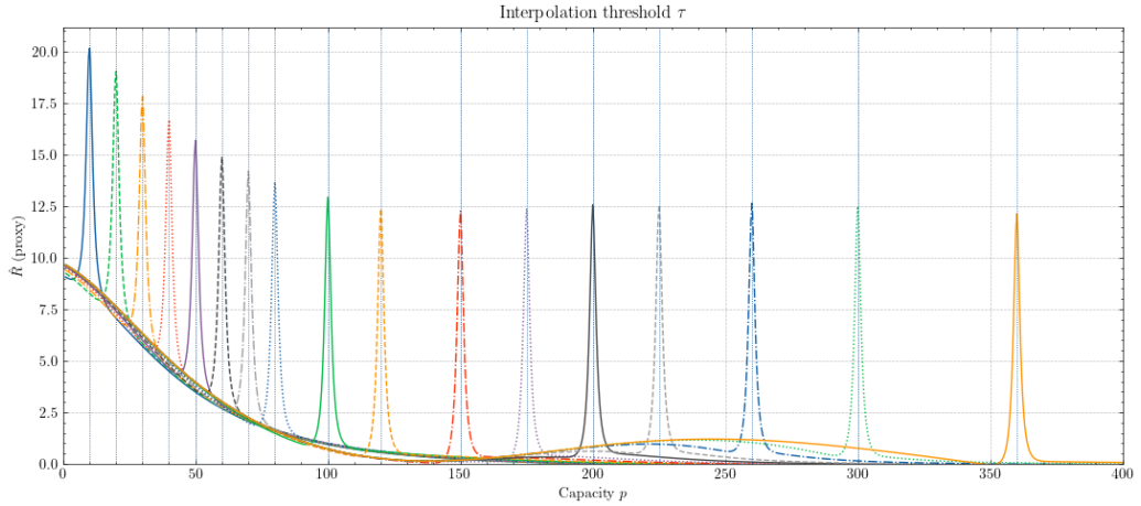
Figure 3.3: Prediction made by certain configurations of Hypothesis 3.2.1. Here, the injected PAC-type decay term provides the global envelope, while the interpolation offset term introduces singular behaviour near capacity-sample equality. The resulting superposition reproduces a family of double-descent-like curves depending on the trajectory in (m, |\mathcal{H}|) -space.
