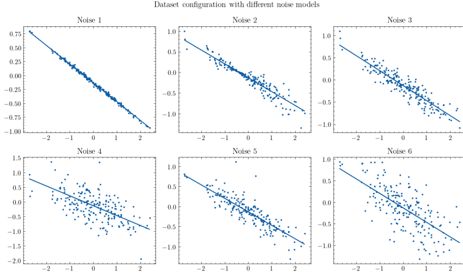
Figure 4.1: The different variations of the noise profile that can be often seen when sampling from a simple regression model. By order, (1) represents mean-scale additive noise, (2) considers heteroskedastic multiplicative noise, (3) considers variance-scaled additive noise, (4) considers absolute additive noise (where scale independent of y ), (5) considers heavy-tailed noise (Student- t modelling), and (6) is the standard canonical Gaussian noise (basically the default). All are under reduced dimension of the simplest linear model on feature space as possible for illustration.
