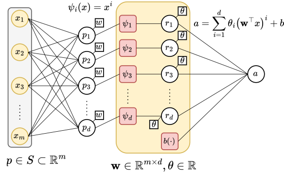
Figure 4.10: Illustration of polynomial model in definition 4.4.2.
