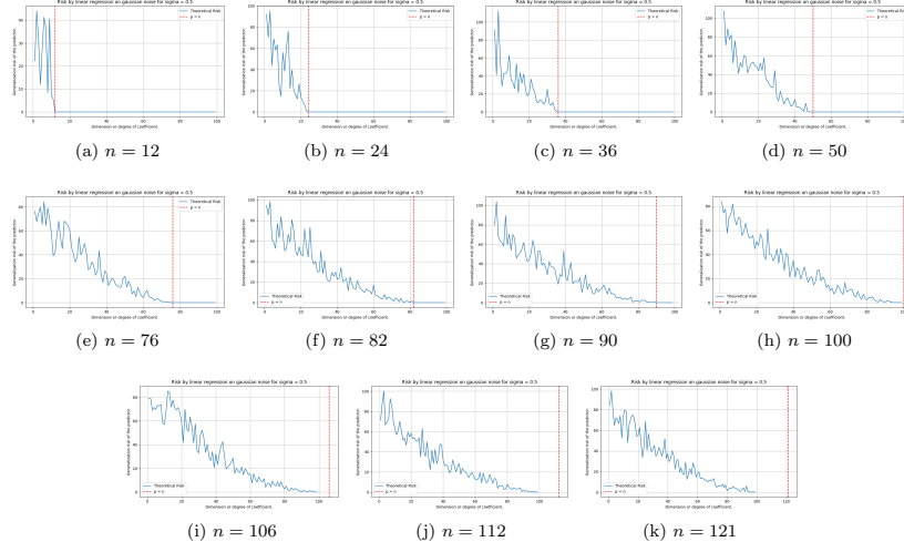
Figure 4.7: Contrary to Theorem 4.3.1 and both figure 4.6, this is the behaviours on randomized setting for standard parameter-wised mean square error measure (MSE-on-prediction). Especially, we do not see double descent pattern in this setting, as it is. For this model, we have d = 100 , \sigma = 0.5 , and variational n . Full test cases are for p = [1, 100] , n = \{12, 24, 36, 50, 76, 82, 90, 100, 106, 112, 121\} accordingly. The test function of the concept itself is the same linear model, but with different input only.
