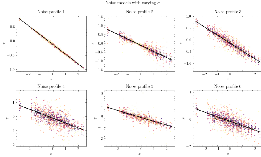
Figure 4.2: The different variations of the noise profile that can be often seen when sampling from a simple regression model, but for different controlling nob for strength of the noise, by \sigma in range of [0.1, 0.2, 0.3, 0.4, 0.5, 0.6] . Again, by order, (1) represents mean-scale additive noise, (2) considers heteroskedastic multiplicative noise, (3) considers variance-scaled additive noise, (4) considers absolute additive noise (where scale independent of y ), (5) considers heavy-tailed noise (Student- t modelling), and (6) is the standard canonical Gaussian noise (basically the default). All are under reduced dimension of the simplest linear model on feature space as possible for illustration.
