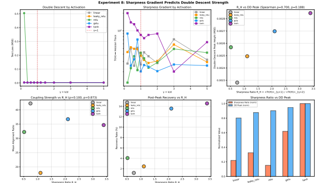
Figure 9. Sharpness Ratio as predictor of double descent. (Top left) Double descent curves for five activations. (Top center) \text{Tr}(H) vs. \gamma on log scale, revealing the sharpness differential. (Top right) DD peak height vs. R_H (Spearman \rho = 0.700 , n = 5 ). (Bottom) Additional diagnostics: coupling vs. R_H , recovery rate, and normalized bar comparison.
