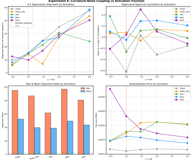
Figure 7. Curvature-noise coupling across five activation functions. (Top left) Eigenvector alignment ratio between H and \Sigma as a function of \gamma . All activations show alignment \gg 1 (random baseline), confirming coupling as a universal property. (Bottom left) Maximum and mean alignment ratio by activation. The linear activation paradoxically exhibits the strongest coupling, despite producing the weakest double descent. (Right) Additional diagnostics: eigenvalue correlation and test error curves.
