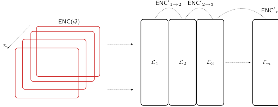
Figure 4.11: Encoding space and the change of encoding inbetween a static graph (or snapshot-wise) GNN. The encoding space is warped toward arbitrary notions inside a GNN, to the point that after certain layers of processing, the encoding outputs different from expected encoding space (native to the model, not to the designer), though there might be universal notions preserved, like the degree of node represented in a different way.
