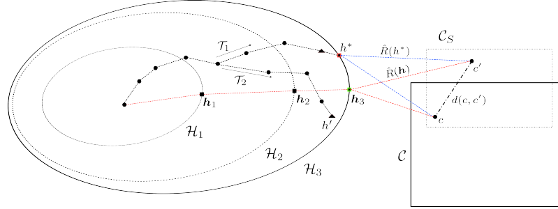
Figure 5.1: Illustrative dynamic of the learning problem. For an incremental hypothesis space sequence \mathcal{H}_1, \mathcal{H}_2, \mathcal{H}_3 , we aim to obtain the procedure \mathcal{T} that would either reach the generalization solution \mathbf{h} , or the empirical solution h^* for a particular hypothesis class, with respect to the concept c and its observed concept c' . Model selection hence dictates how an algorithm or procedure than choose the best possible hypothesis to approximate the generalization solution from the empirical solution set. Do notice that here we explicitly state that the data would create a proxy concept that overlaps with the concept class and of some arbitrary 'distance' from the true concept by d(c, c') . In case the two classes overlap, there still exists the arbitrary distance. Also, we can also observe the intuitive notion of increasing hypothesis class - while it indeed can help in getting closer to the concept class, the somewhat intrinsic property of current learning theory being the relative random procedure class make it probabilistically unstable.
