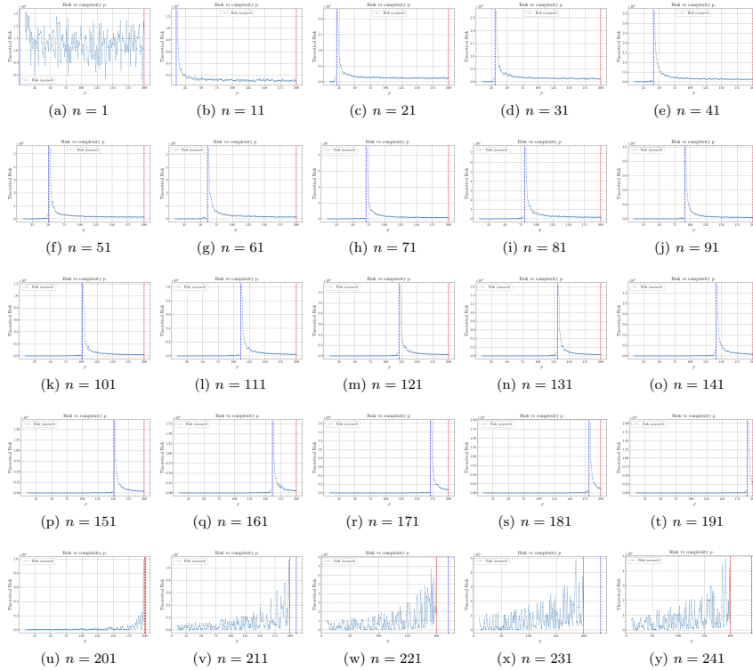
Figure 4.5: Extension general experimentation, using the prediction made of theorem 4.1.1 for verification. Here, q = 1 as the general basis case of verification.
