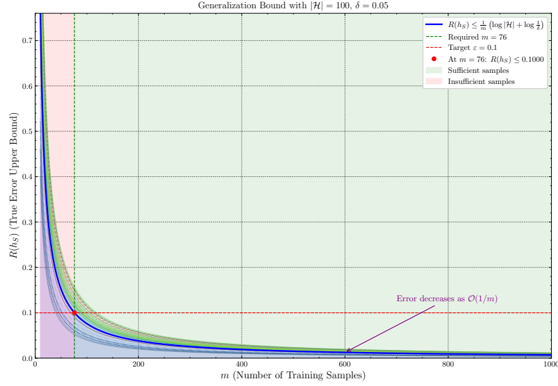
Figure 3.2: Illustration of generalizational error/risk in terms of cardinality m = |S| , with respect to changing \mathcal{H} cardinality and \delta -value measure. Blurred line indicates different cases or values, the deviation is rather small, thus the bound is very tight.
