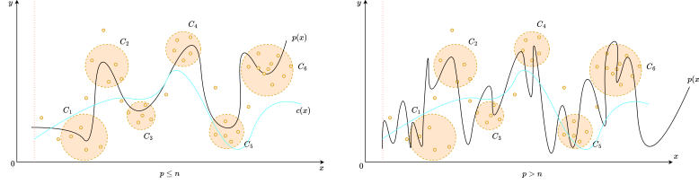
Figure 4.7: Intuition of Hypothesis 4.2.1. Effectively, in the overparametrized range ( p > n ), the problem turns into soft interpolation, where the polynomial is possible to be dense enough such that relative error remains internally low. This can also happen if the dataset itself is intrinsically large.
