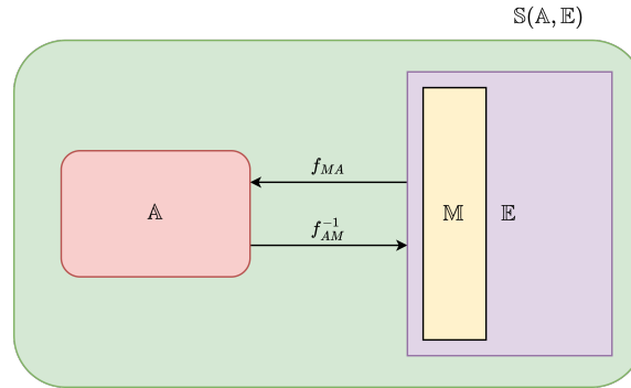
Figure 6.1: Illustration of ambience and encoding space, alongside a specific structural compact on the encoding. The notation shifted to \mathcal{A}, \mathcal{M}, \mathcal{E} , but nevertheless represents the same structure. Here, as we can see, the system space contains ambience and encoding space, alongside a specific encoding-related structure \mathcal{M} , and then two decoding and encoding which is short for interpreting between the two encoding spaces.
