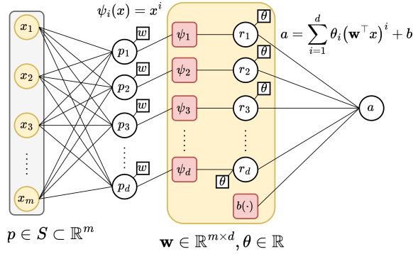
Figure 4.8: Illustration of polynomial model in definition 4.2.7.
