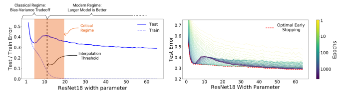
Figure 6. Left: Train and test error as a function of model size, for ResNet18s of varying width on CIFAR-10 with 15% label noise. Right: Test error, shown for varying train epochs. All models trained using Adam for 4K epochs. The largest model (width 64) corresponds to standard ResNet18. Reused from Nakkiran et al. 2019.
