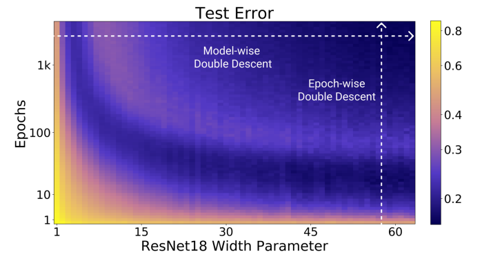
Figure 7. Test error as a function of model size and train epochs. The horizontal line corresponds to model-wise double descent—varying model size while training for as long as possible. The vertical line corresponds to epoch-wise double descent, with test error undergoing double-descent as train time increases. Reused from Nakkiran et al. 2019
