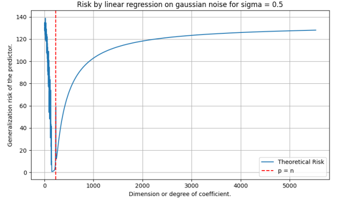
Figure 12. Similar experiment according to setting and result of Theorem 61, where p is in the range [1, 5523] . Here, we can see small double descent modelled exactly at the interpolation threshold, while the later region exhibit similar phenomenon as bias-variance tradeoff.
