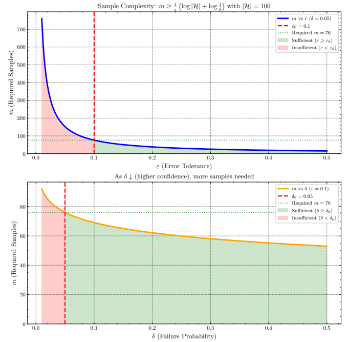
Figure 1. Illustration of of sample complexity in terms of cardinality m = |S| , with respect to \epsilon or \delta measure.
