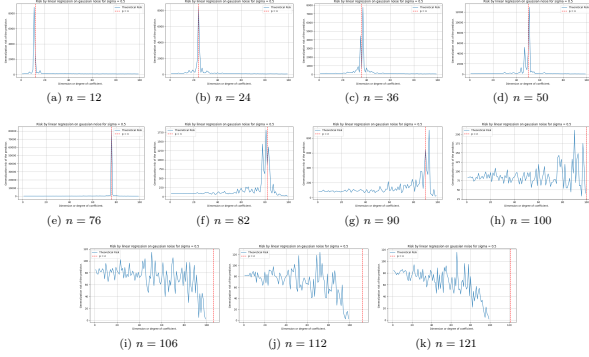
Figure 10. Contrary to Theorem 8.1, this is the behaviours on randomized setting for standard parameter-wise mean square error measure (MSE-on-parameter). For this model, we have d = 100 , \sigma = 0.5 , and variational n . Full test cases are for p = [1, 100] , n = \{12, 24, 36, 50, 76, 82, 90, 100, 106, 112, 121\} accordingly. The test function of the concept itself is the same linear model, but with different input only.
