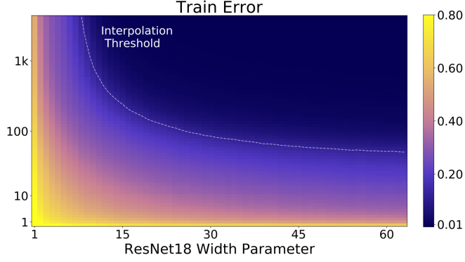
Figure 8. Train error of the corresponding models. All models are Resnet18s trained on CIFAR-10 with 15% label noise, data-augmentation, and Adam for up to 4K epochs. Reused from Nakkiran et al. 2019
