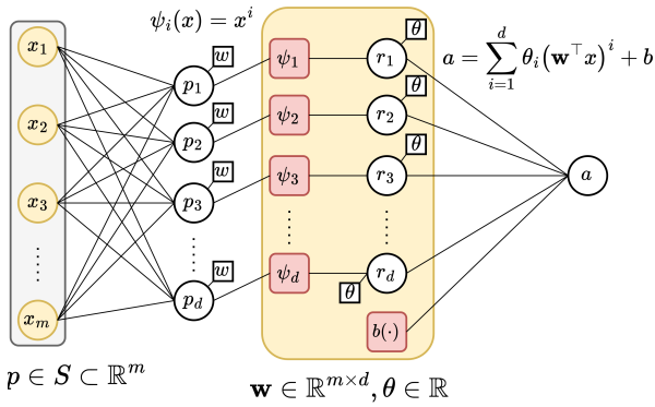
Figure 15. Illustration of polynomial model in definition 9.7.
