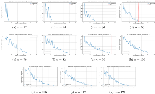
Figure 11. Contrary to Theorem 8.1 and both figure 10, this is the behaviours on randomized setting for standard parameter-wise mean square error measure (MSE-on-prediction). Especially, we do not see double descent pattern in this setting, as it is. For this model, we have d = 100 , \sigma = 0.5 , and variational n . Full test cases are for p = [1, 100] , n = \{12, 24, 36, 50, 76, 82, 90, 100, 106, 112, 121\} accordingly. The test function of the concept itself is the same linear model, but with different input only.
