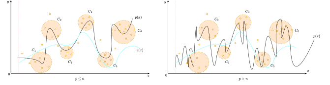
Figure 14. Intuition of Hypothesis 9.1. Effectively, in the overparameterized range ( p > n ), the problem turns into soft interpolation, where the polynomial is possible to be dense enough such that relative error remains internally low. This can also happen if the dataset itself is intrinsically large.
