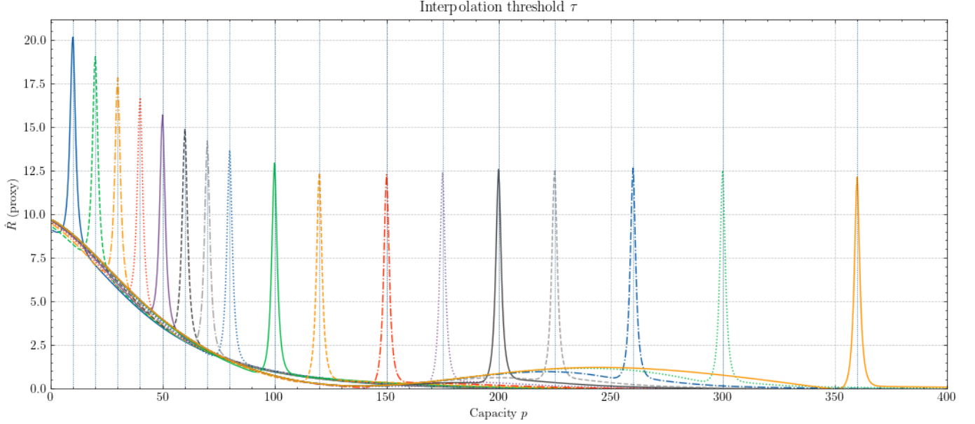
Figure 3. Prediction made by certain configurations of Hypothesis 3.1.
