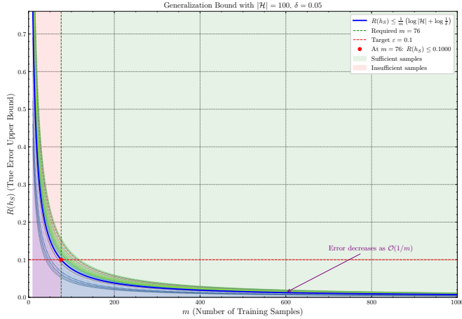
Figure 2. Illustration of of generalizational error/risk in terms of cardinality m = |S| , with respect to changing \mathcal{H} cardinality and \delta -value measure. Blurred line indicates different cases or values, the deviation is rather small, thus the bound is very tight.
