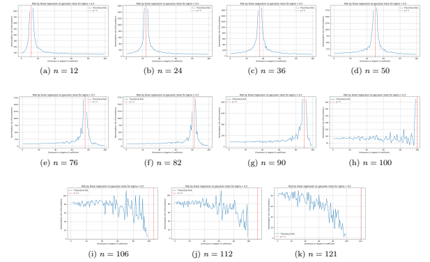
Figure 9. Theorem 8.1 behaviours on randomized setting. For this model, we have d = 100 , \sigma = 0.5 , and variational n . Full test cases are for p = \llbracket 1, 100 \rrbracket , n = \{12, 24, 36, 50, 76, 82, 90, 100, 106, 112, 121\} accordingly. The test function of the concept itself is the same linear model, but with different input only.
