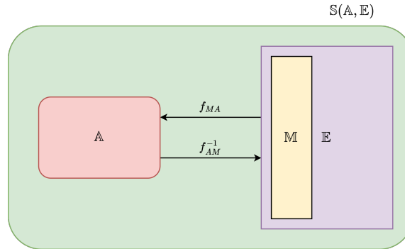
Figure 6.1: Illustration of ambiance and encoding space , alongside a specific structural compact on the encoding. The notation shifted to \mathcal{A}, \mathcal{M}, \mathcal{E} , but nevertheless represents the same structure. Here, as we can see, the system space contains ambiance and encoding space , alongside a specific encoding-related structure \mathcal{M} , and then two decoding and encoding which is short for interpreting between the two encoding spaces.
