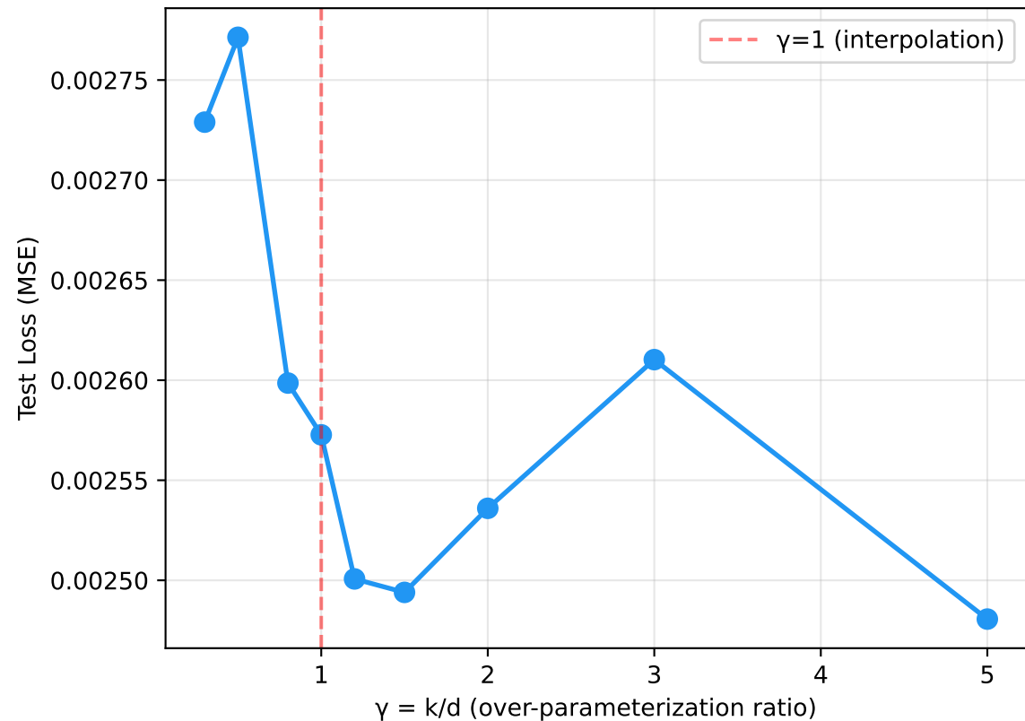
Double Descent: Test Error vs \gamma
