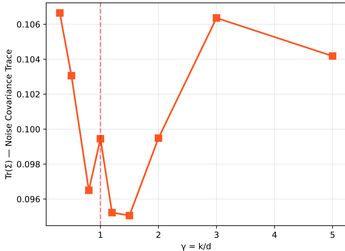
Noise Amplification at Interpolation Threshold
