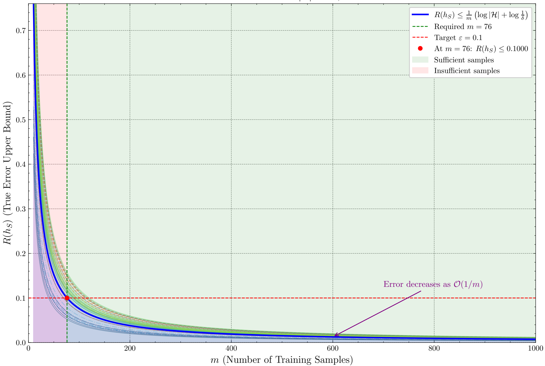
Generalization Bound with |\mathcal{H}| = 100 , \delta = 0.05
